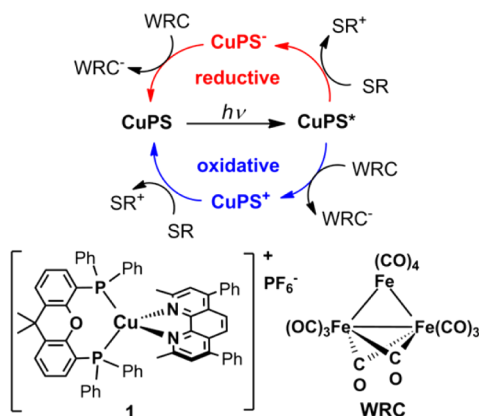
Scheme 1. Reductive (red) and Oxidative (blue) Reaction Pathway and the Initial Structures of the Applied Copper Photosensitizer (CuPS, e.g., 1) and Water Reduction (WRC)
