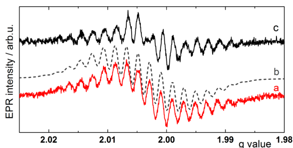
Figure 1. EPR spectra of (a) CuPS 1 in THF/TEA (4/1) under UV/vis irradiation, (b) the respective EPR simulation ( g = 2.0034 , line width \Delta B = 2.5\text{G} , 2 \times A_{\text{H}} = 10.0\text{G} , 2 \times A_{\text{H}} = 7.0\text{G} , 2 \times A_{\text{N}} = 3.4\text{G} , 1 \times A_{\text{Cu}} = 3.4\text{G} ), and (c) I – obtained at -1.5\text{ V vs Ag/Ag}^+ .
