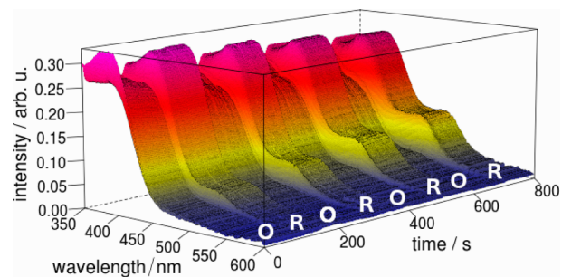
Figure 2. Oxidation (O, +1.5\text{ V} ) and reduction (R, at -0.5\text{ V vs Ag/Ag}^+ ) cycles (duration of each step: 100 s) of 1 in acetonitrile solution monitored by UV/vis spectroelectrochemistry.
